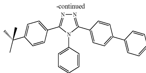
TAZ
