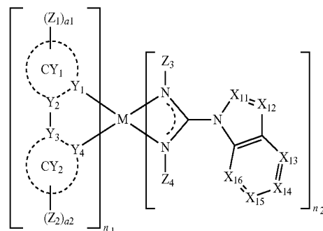
Formula 1C
