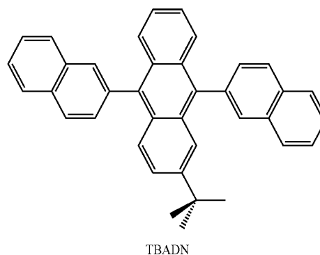
TBADN
